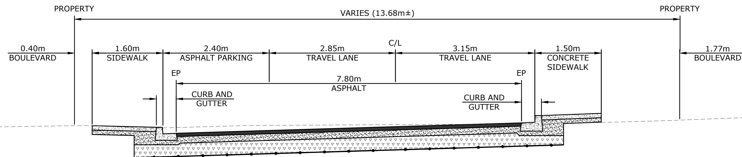
C-C 001A SCALE: 1:50 TYPICAL SECTION STA. 0+150 TO 0+210
